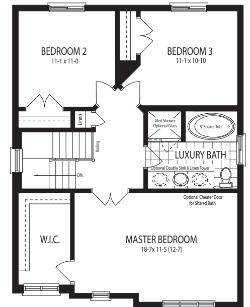
Second Floor Optional Master Bedroom Layout
